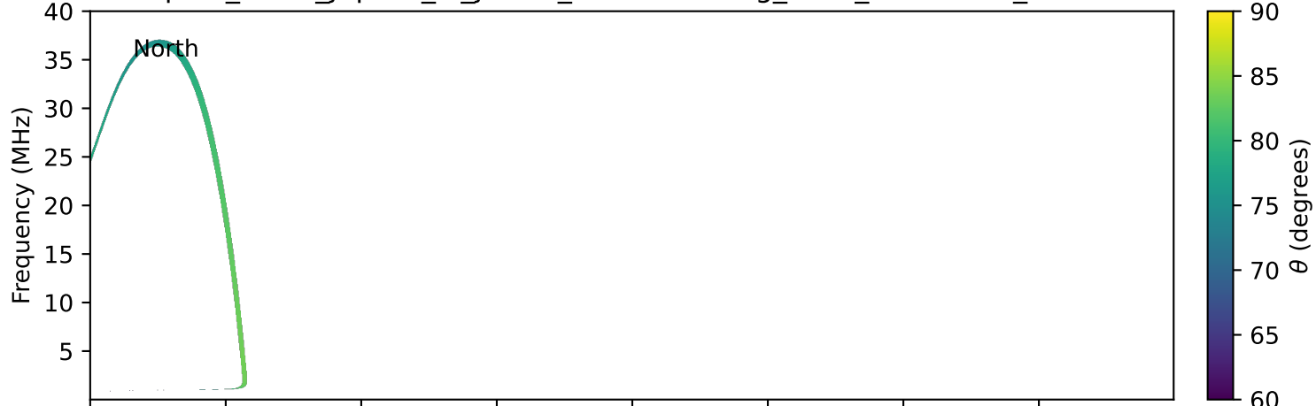
expres_earth_jupiter_io_jrm33_lossc-wid1deg_3kev_20200819_v11.cdf
