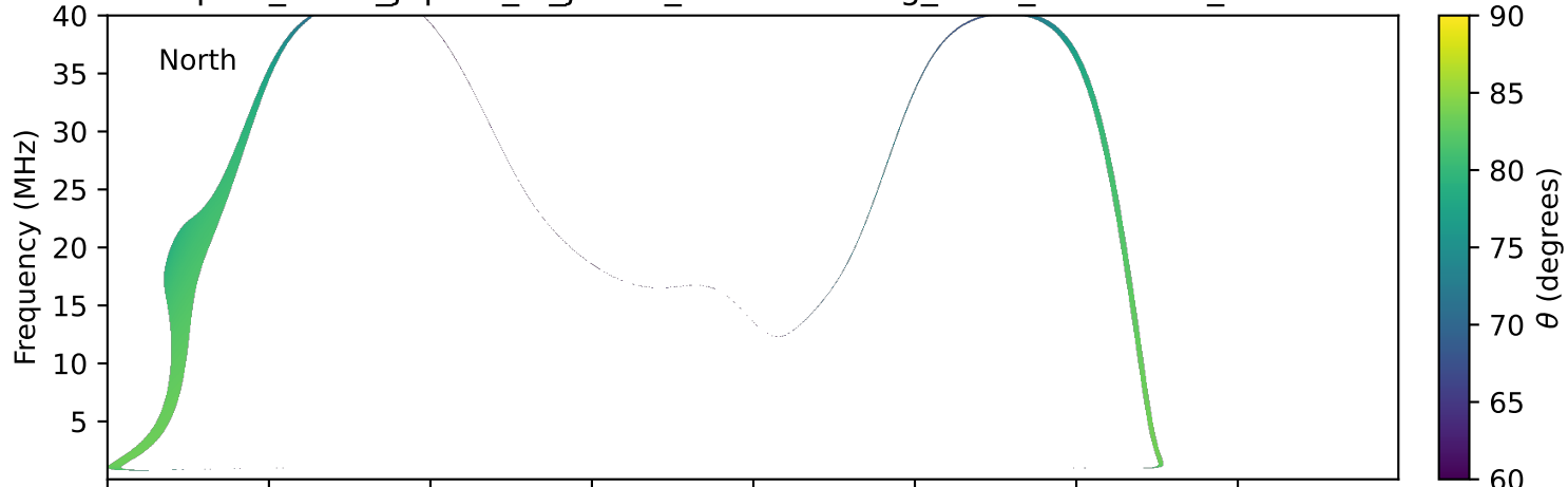
expres_earth_jupiter_io_jrm33_lossc-wid1deg_3kev_20200813_v11.cdf
