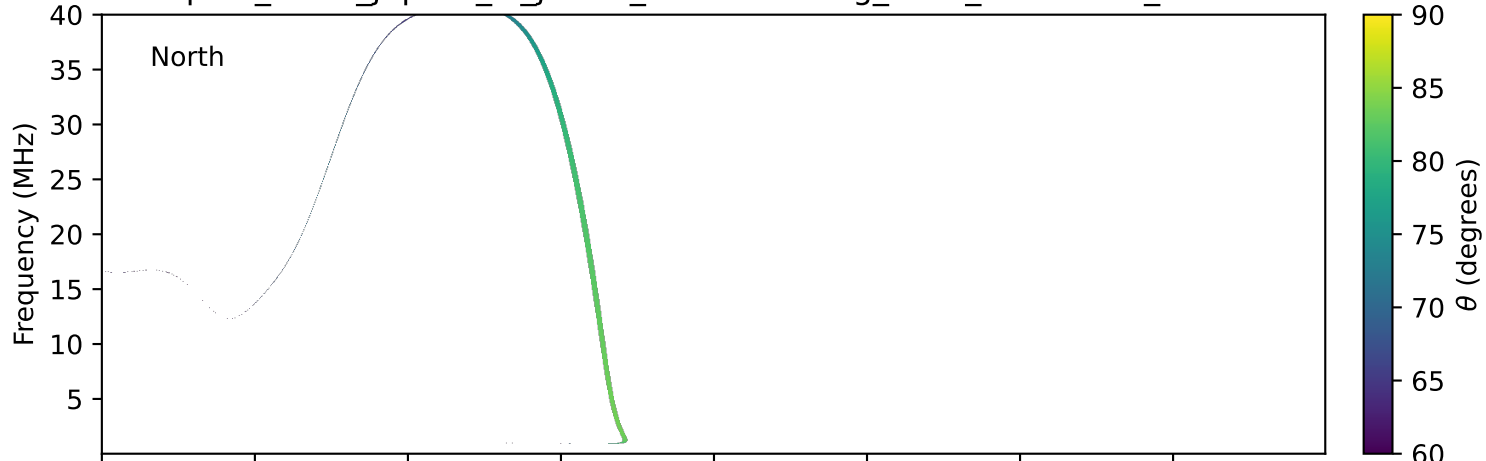
expres_earth_jupiter_io_jrm33_lossc-wid1deg_3kev_20200801_v11.cdf
