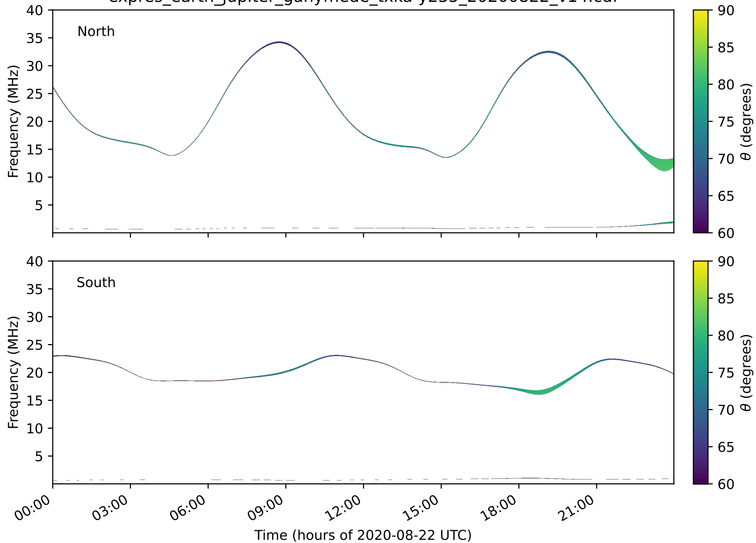
expres_earth_jupiter_ganymede_txka-y235_20200822_v14.cdf
