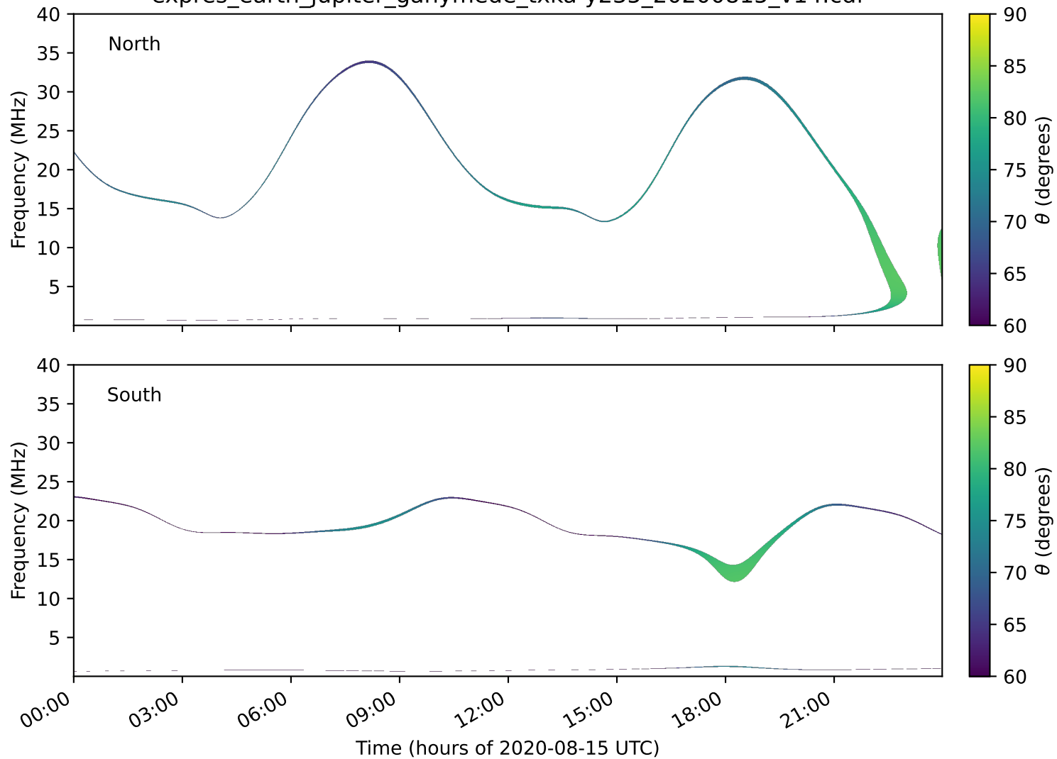
expres_earth_jupiter_ganymede_txka-y235_20200815_v14.cdf
