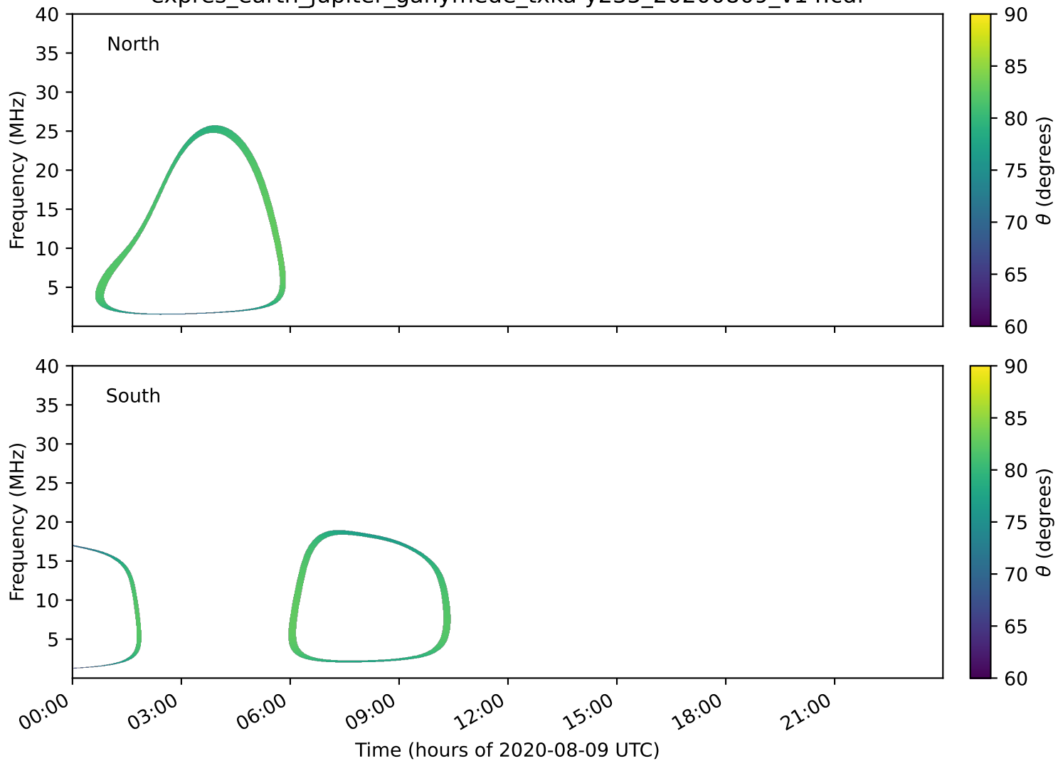
expres_earth_jupiter_ganymede_txka-y235_20200809_v14.cdf
