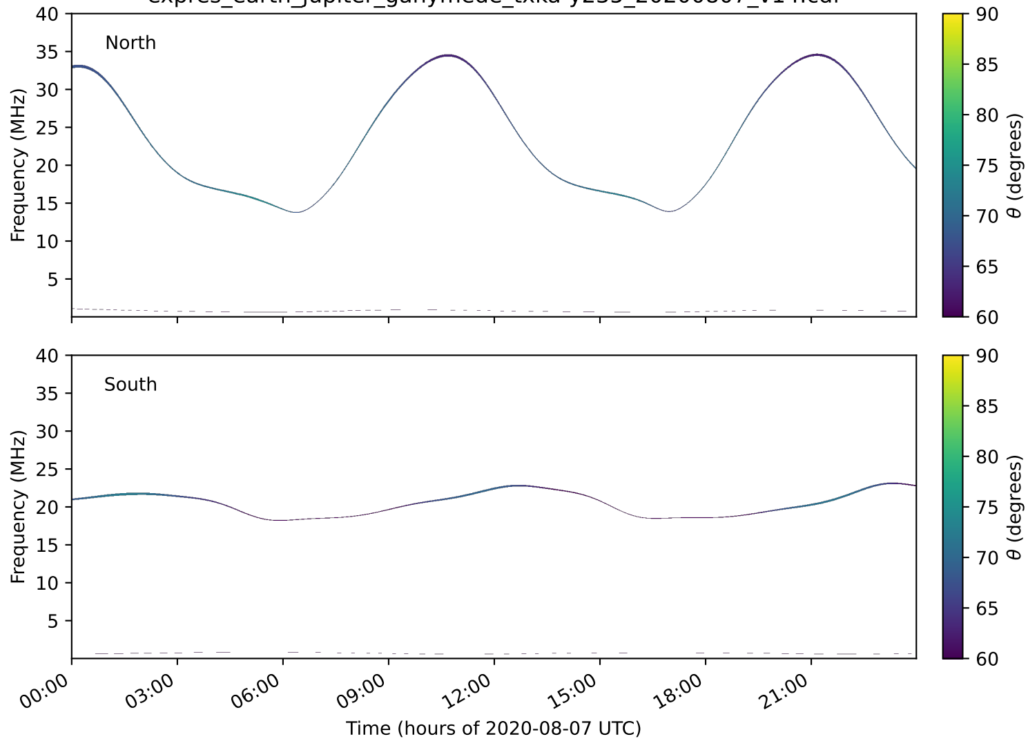
expres_earth_jupiter_ganymede_txka-y235_20200807_v14.cdf
