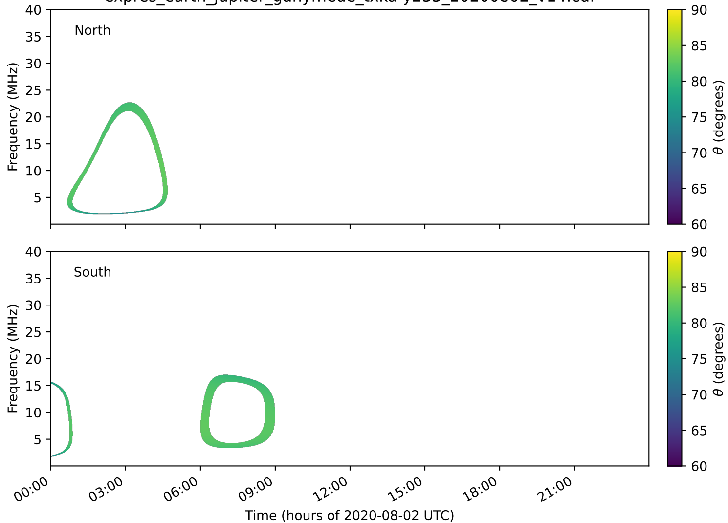
expres_earth_jupiter_ganymede_txka-y235_20200802_v14.cdf
