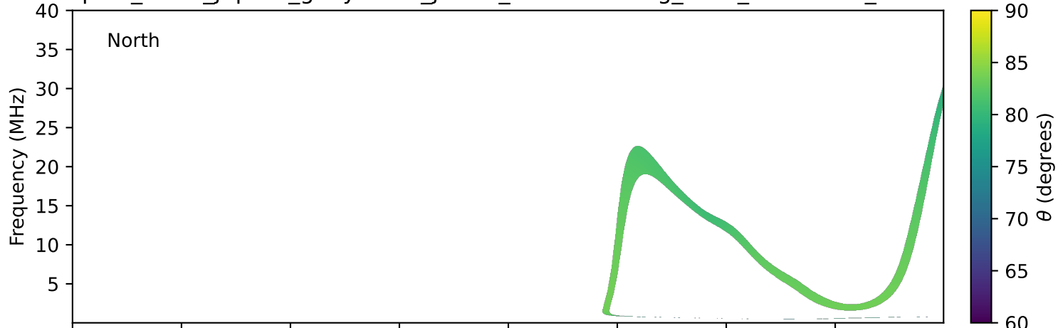
expres_earth_jupiter_ganymede_jrm33_lossc-wid1deg_3kev_20200820_v11.cdf
