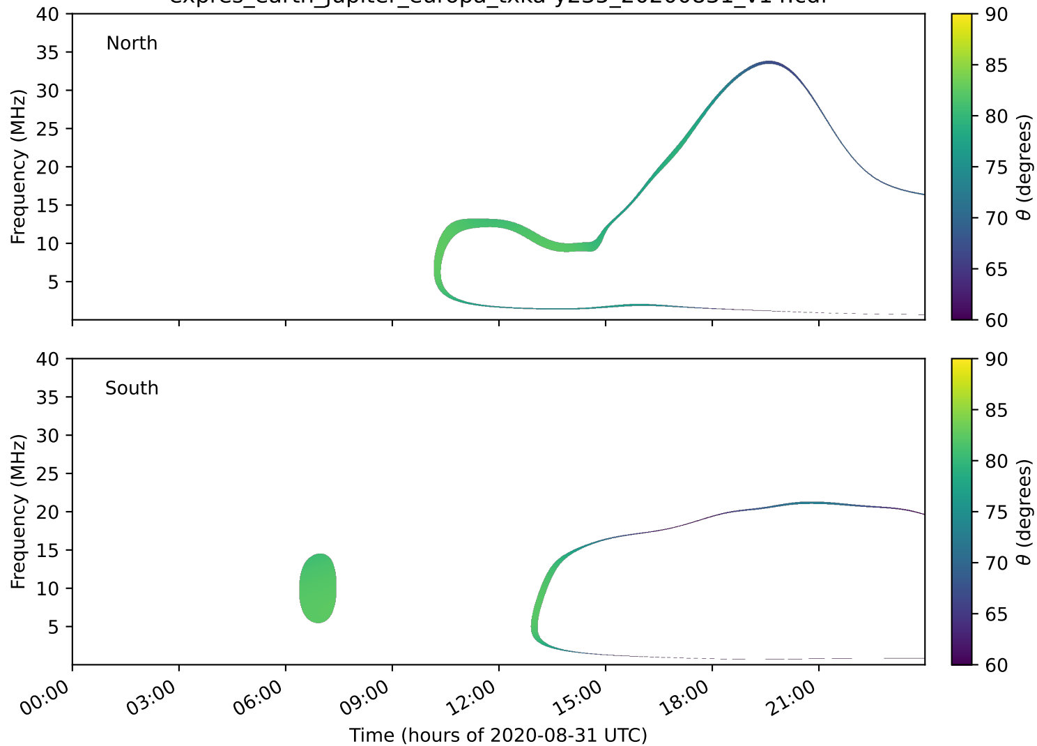
expres_earth_jupiter_europa_txka-y235_20200831_v14.cdf
