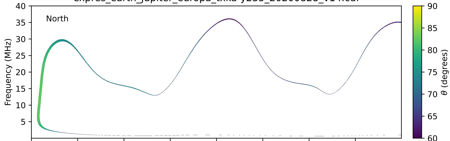
expres_earth_jupiter_europa_txka-y235_20200828_v14.cdf
