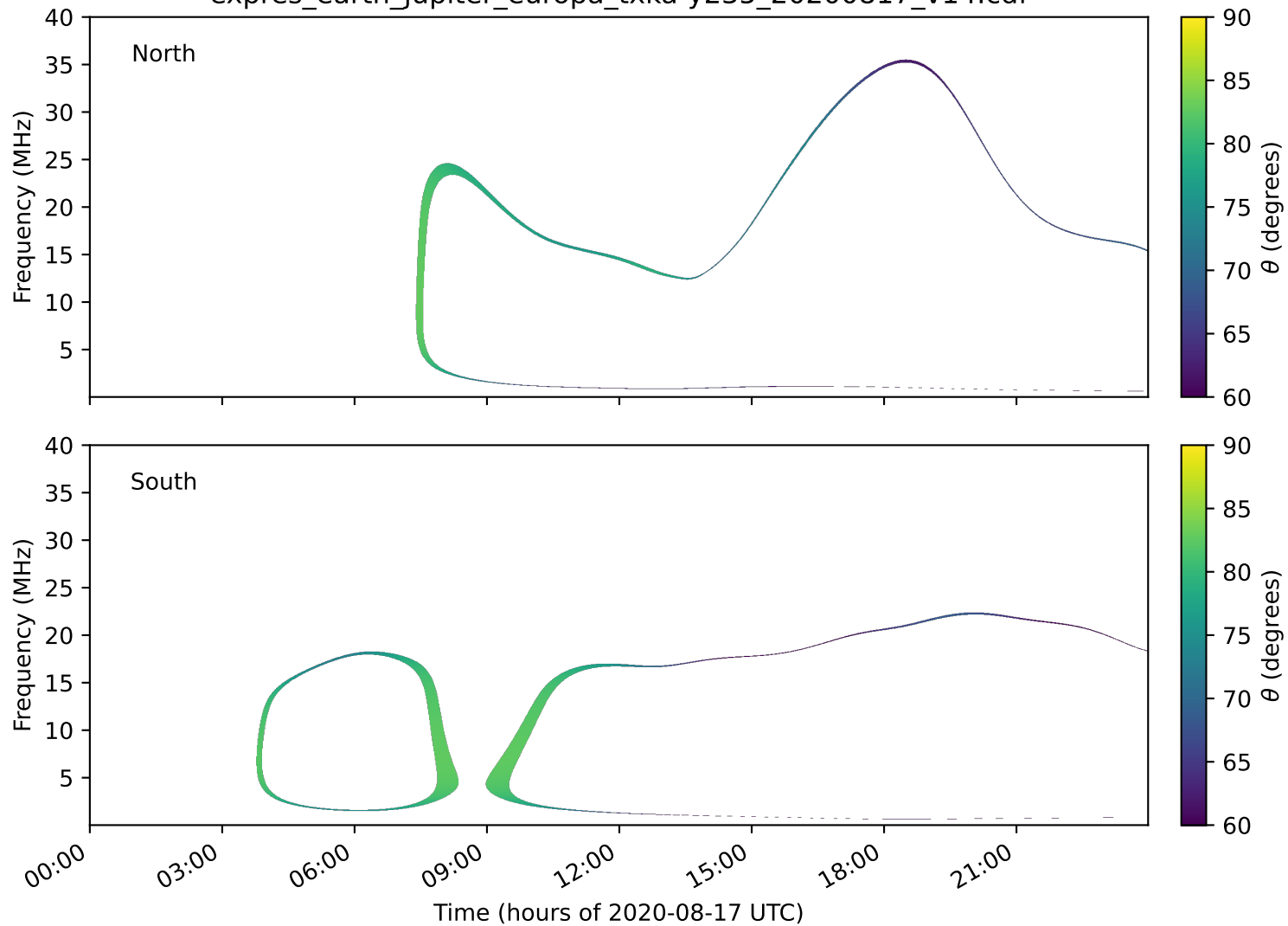
expres_earth_jupiter_europa_txka-y235_20200817_v14.cdf
