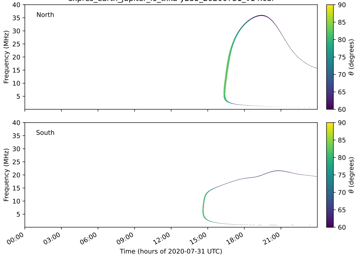
expres_earth_jupiter_io_txka-y235_20200731_v14.cdf
