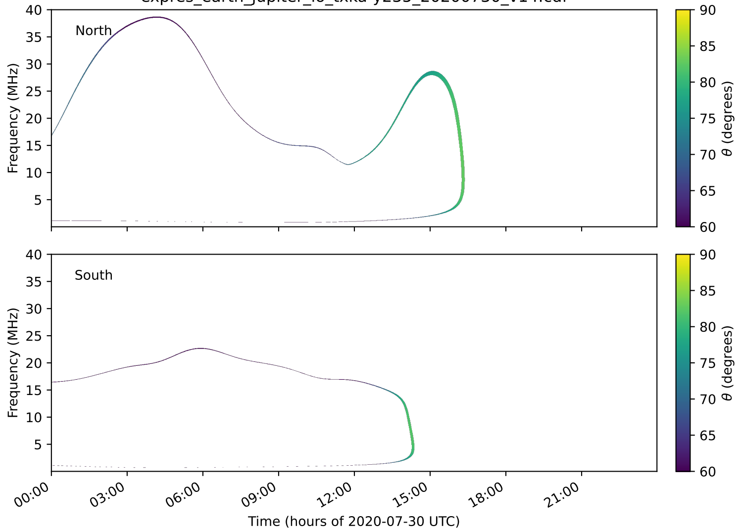
expres_earth_jupiter_io_txka-y235_20200730_v14.cdf
