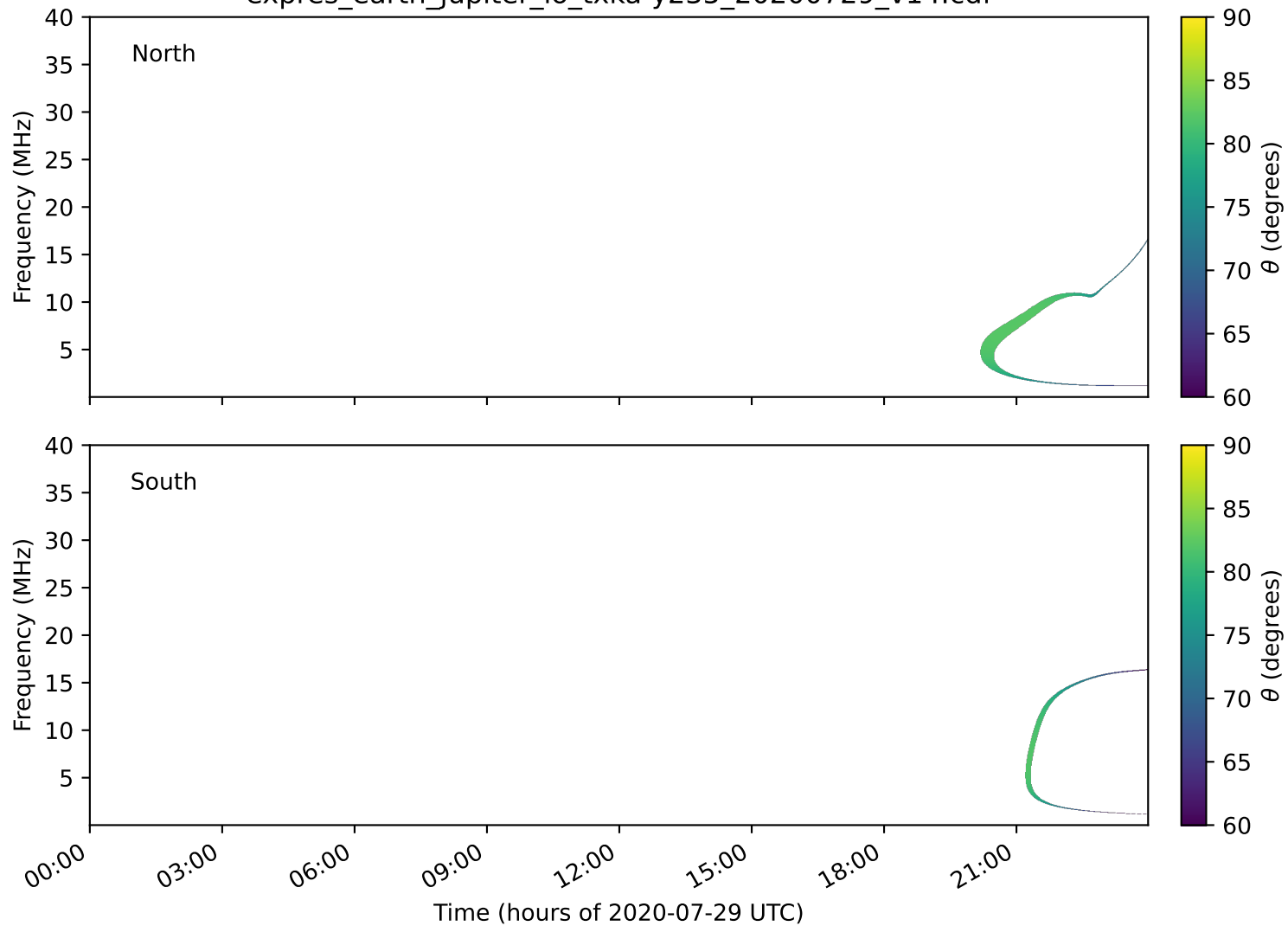
expres_earth_jupiter_io_txka-y235_20200729_v14.cdf
