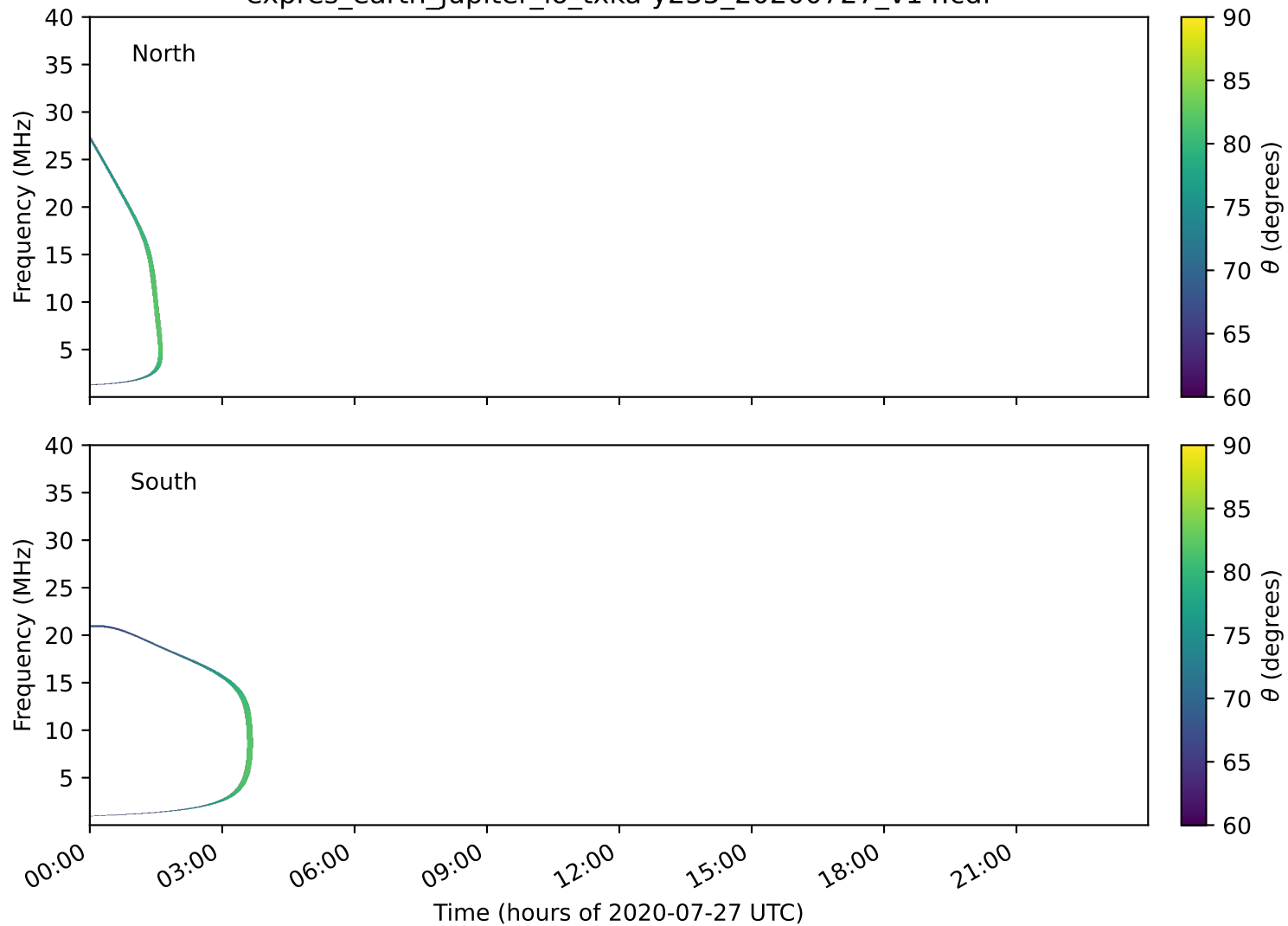
expres_earth_jupiter_io_txka-y235_20200727_v14.cdf
