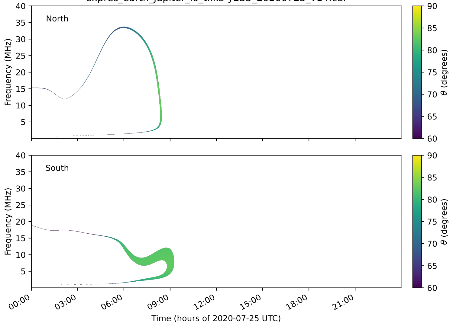
expres_earth_jupiter_io_txka-y235_20200725_v14.cdf
