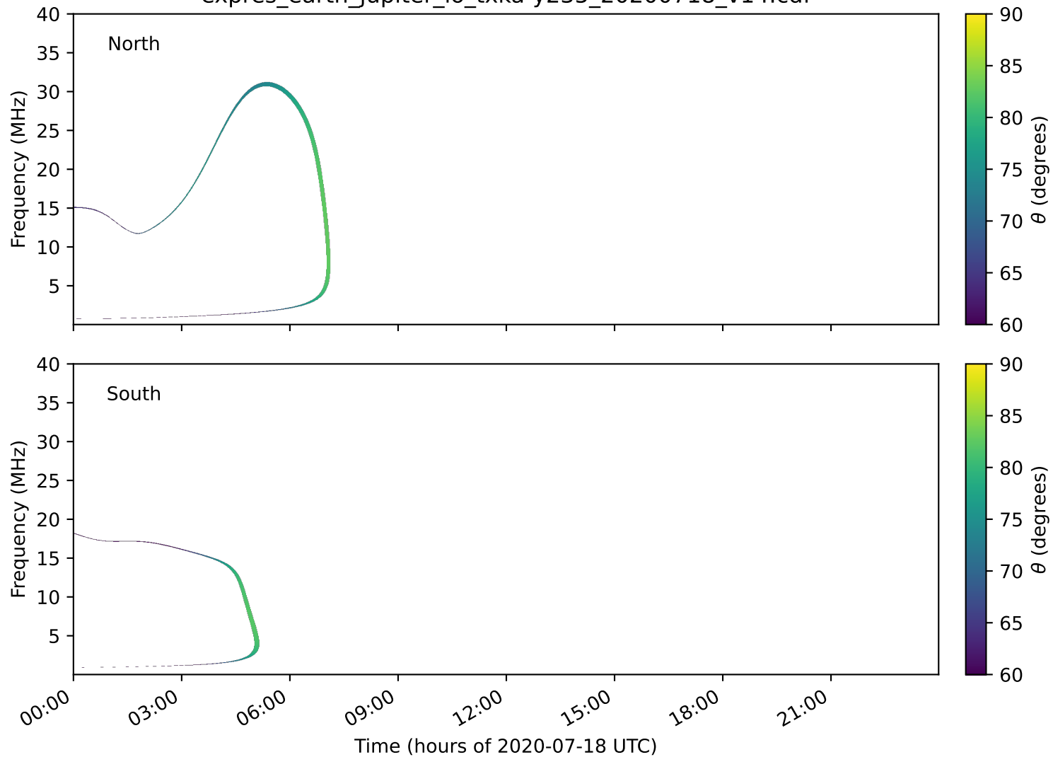
expres_earth_jupiter_io_txka-y235_20200718_v14.cdf
