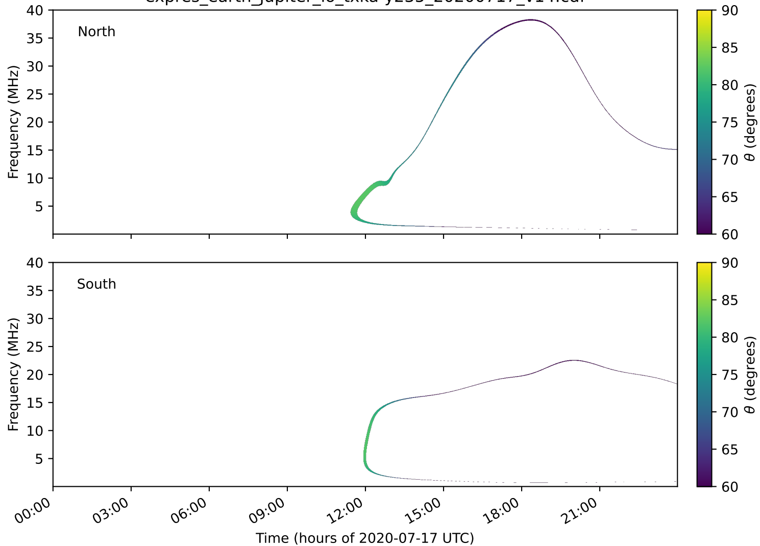
expres_earth_jupiter_io_txka-y235_20200717_v14.cdf
