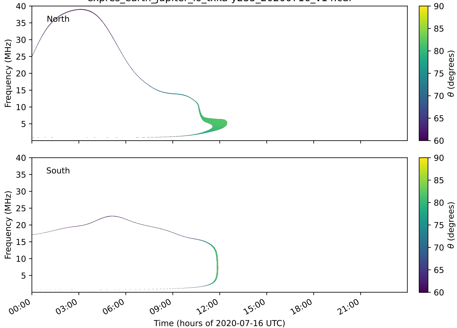
expres_earth_jupiter_io_txka-y235_20200716_v14.cdf
