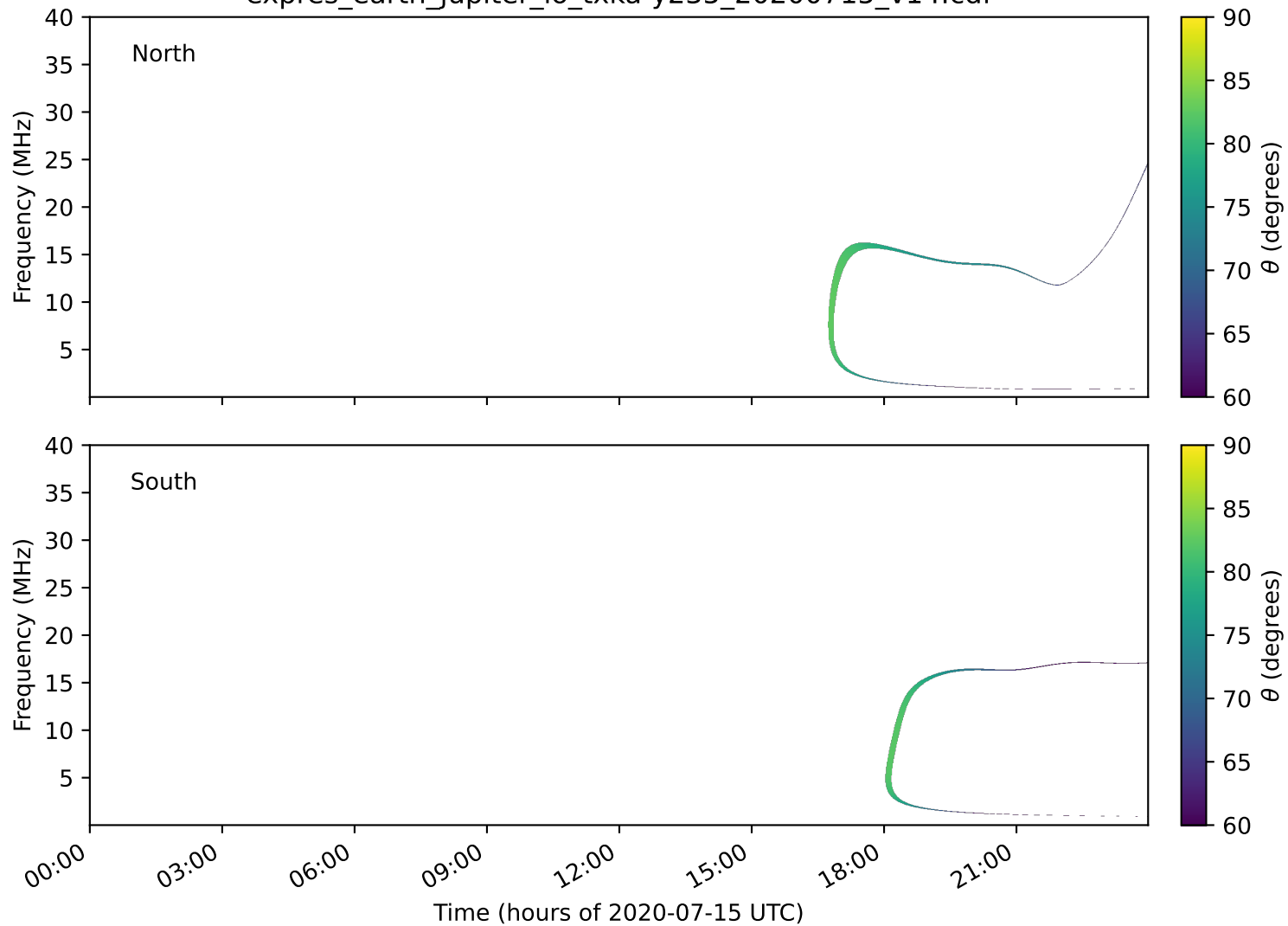
expres_earth_jupiter_io_txka-y235_20200715_v14.cdf
