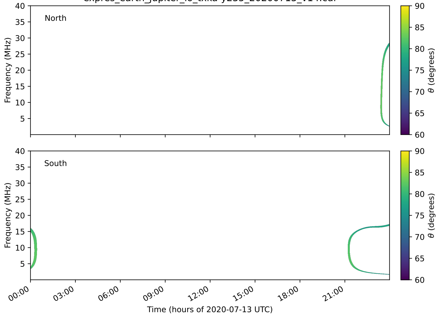
expres_earth_jupiter_io_txka-y235_20200713_v14.cdf
