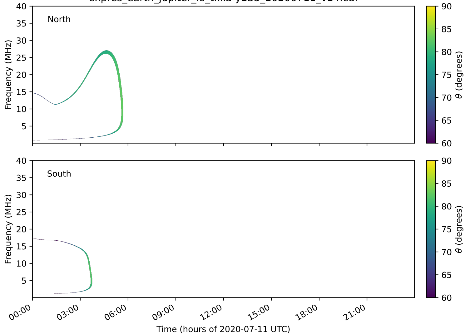
expres_earth_jupiter_io_txka-y235_20200711_v14.cdf
