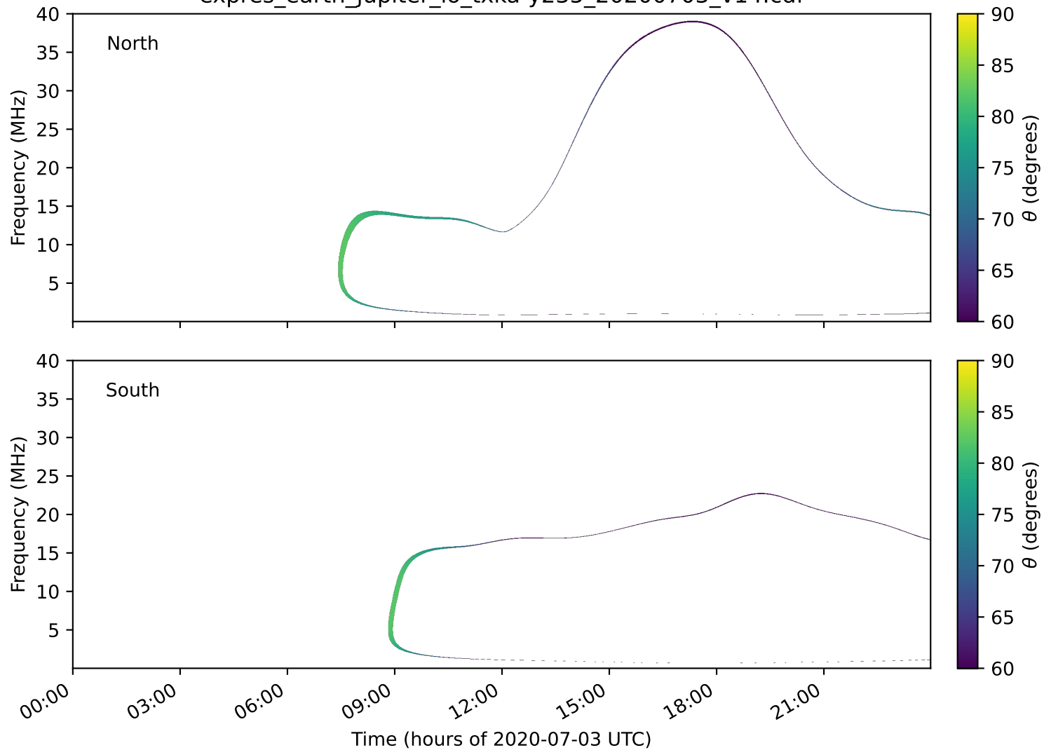
expres_earth_jupiter_io_txka-y235_20200703_v14.cdf
