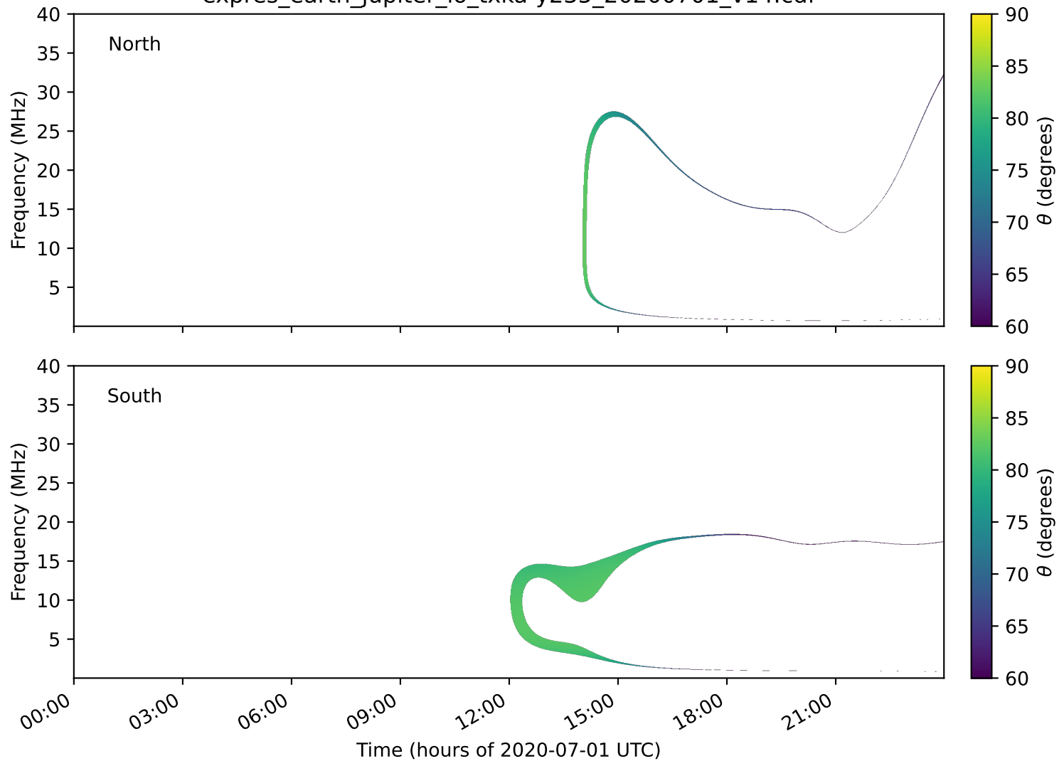
expres_earth_jupiter_io_txka-y235_20200701_v14.cdf
