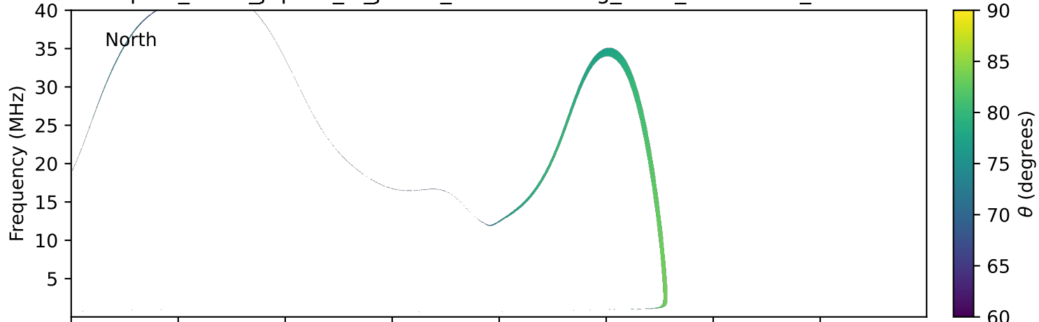
expres_earth_jupiter_io_jrm33_lossc-wid1deg_3kev_20200730_v11.cdf
