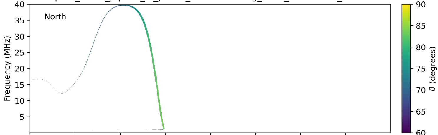
expres_earth_jupiter_io_jrm33_lossc-wid1deg_3kev_20200725_v11.cdf
