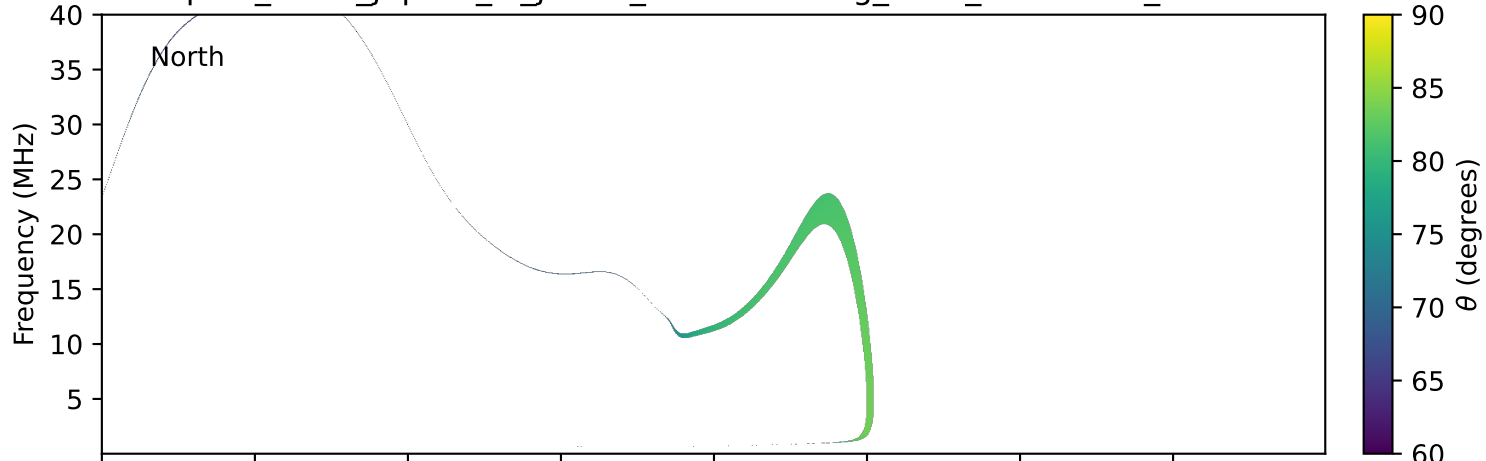
expres_earth_jupiter_io_jrm33_lossc-wid1deg_3kev_20200723_v11.cdf
