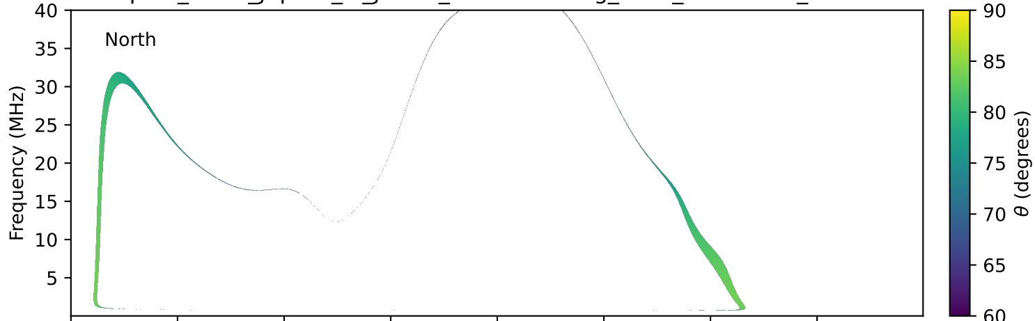
expres_earth_jupiter_io_jrm33_lossc-wid1deg_3kev_20200721_v11.cdf
