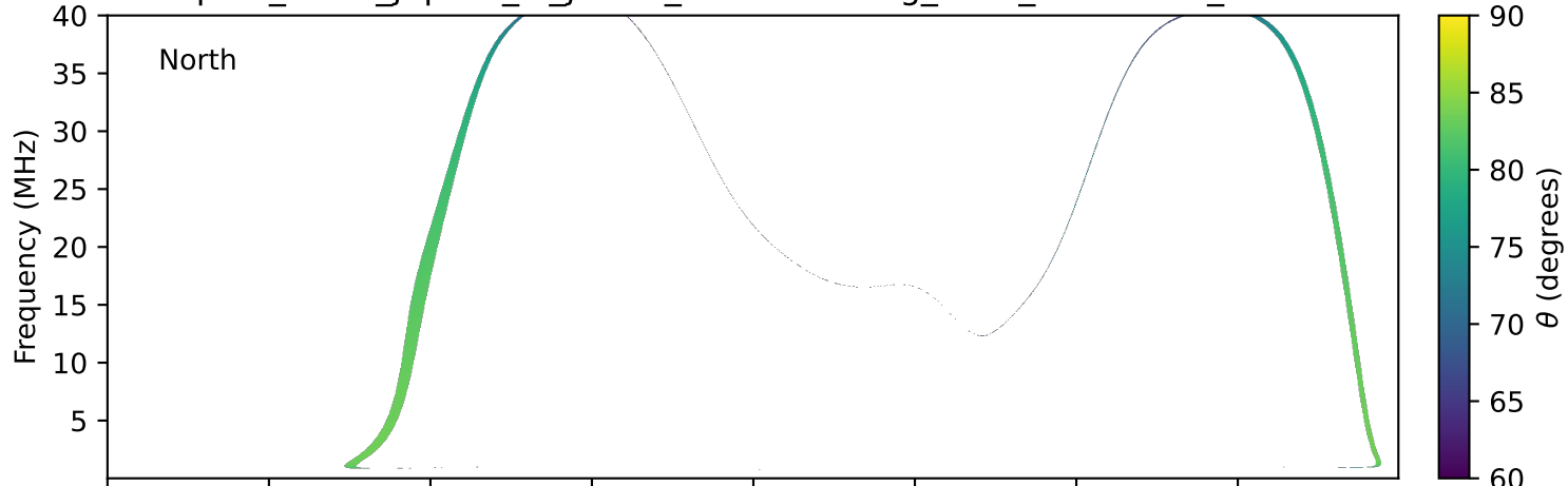
expres_earth_jupiter_io_jrm33_lossc-wid1deg_3kev_20200712_v11.cdf
