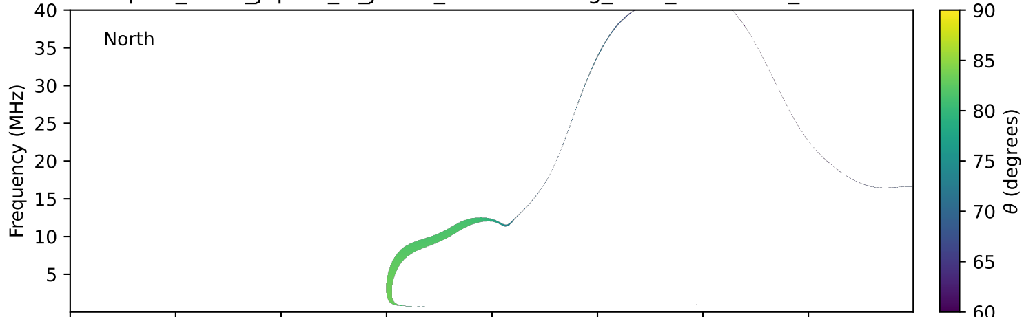
expres_earth_jupiter_io_jrm33_lossc-wid1deg_3kev_20200710_v11.cdf
