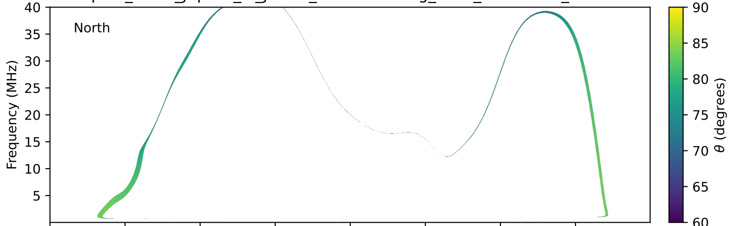
expres_earth_jupiter_io_jrm33_lossc-wid1deg_3kev_20200705_v11.cdf
