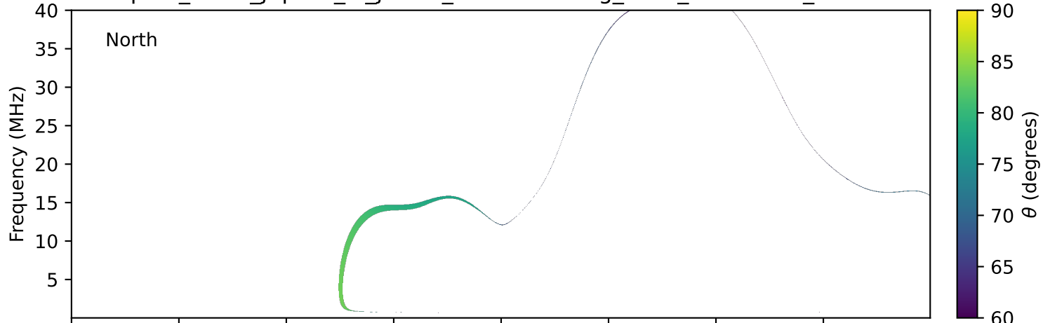
expres_earth_jupiter_io_jrm33_lossc-wid1deg_3kev_20200703_v11.cdf
