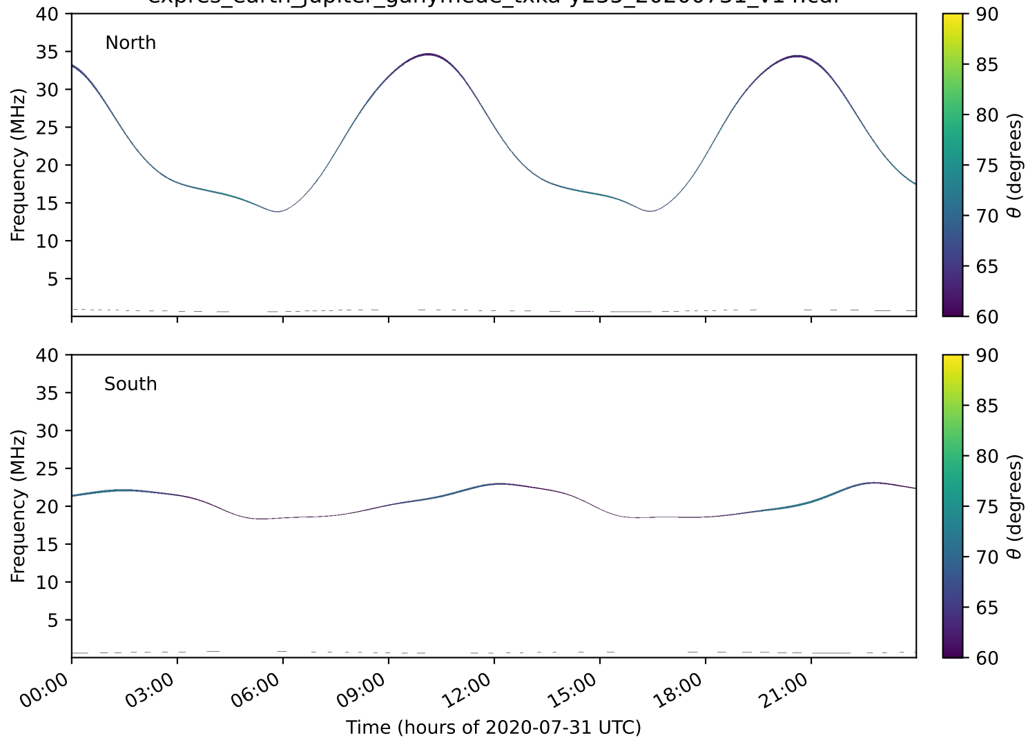
expres_earth_jupiter_ganymede_txka-y235_20200731_v14.cdf
