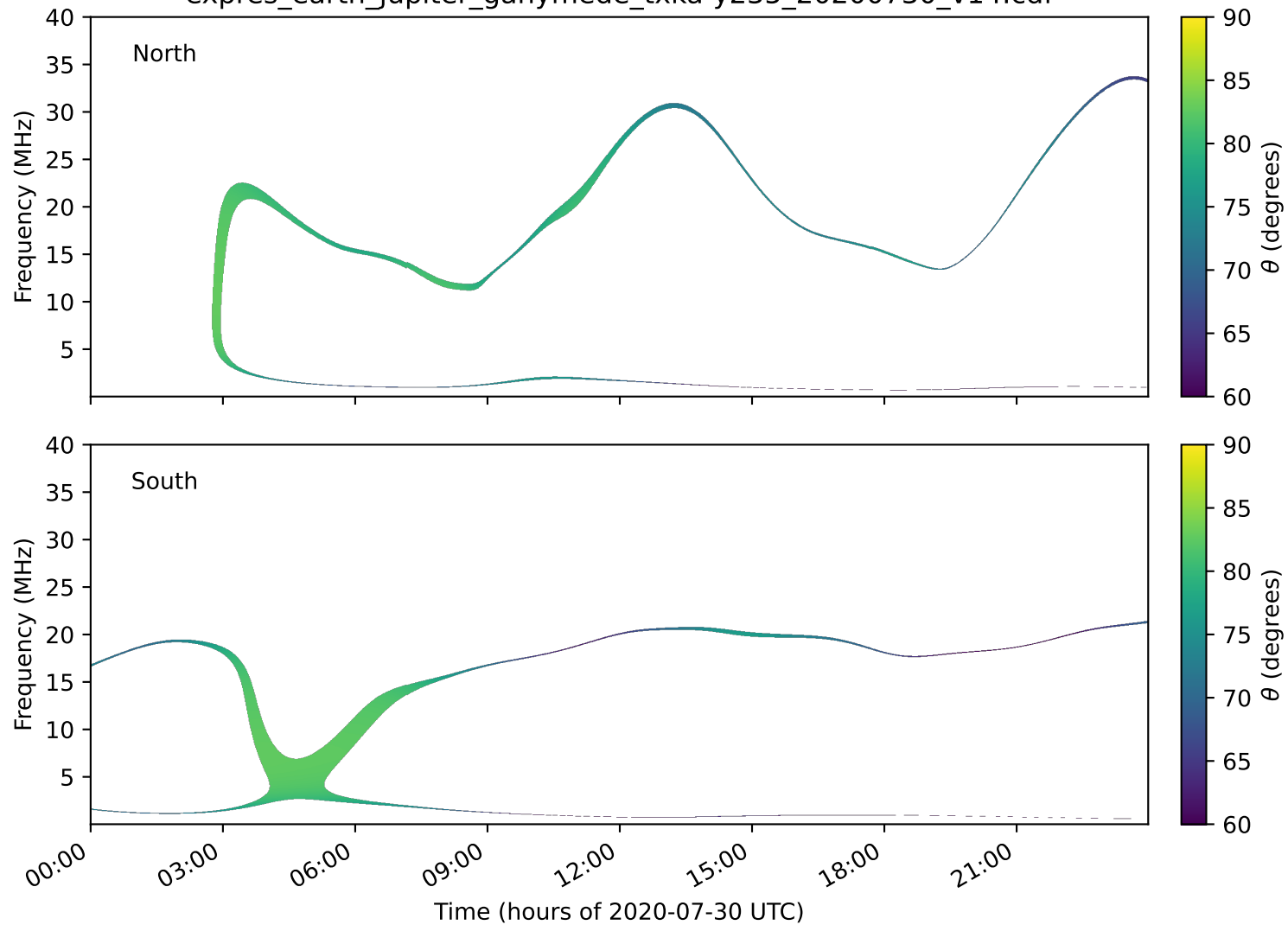
expres_earth_jupiter_ganymede_txka-y235_20200730_v14.cdf
