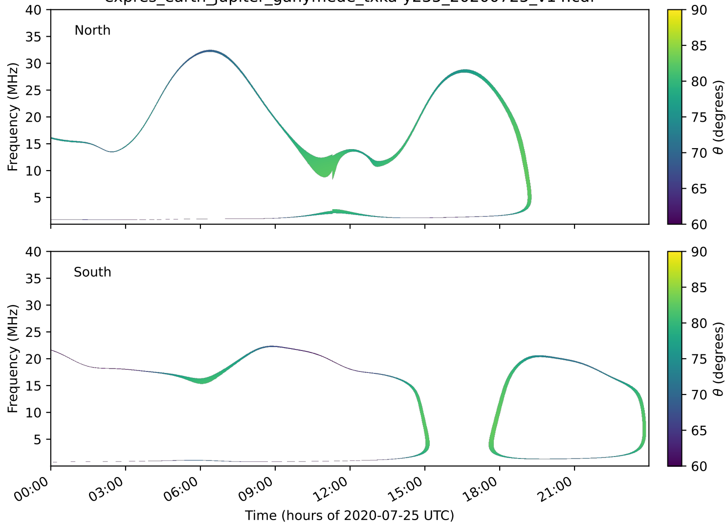
expres_earth_jupiter_ganymede_txka-y235_20200725_v14.cdf
