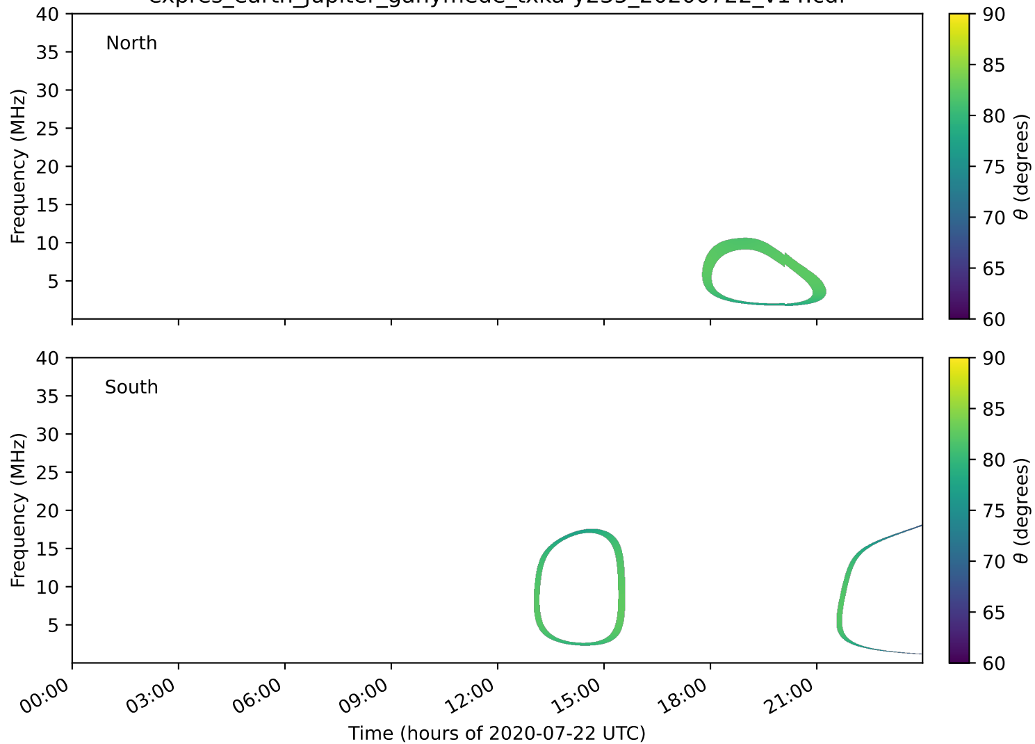
expres_earth_jupiter_ganymede_txka-y235_20200722_v14.cdf
