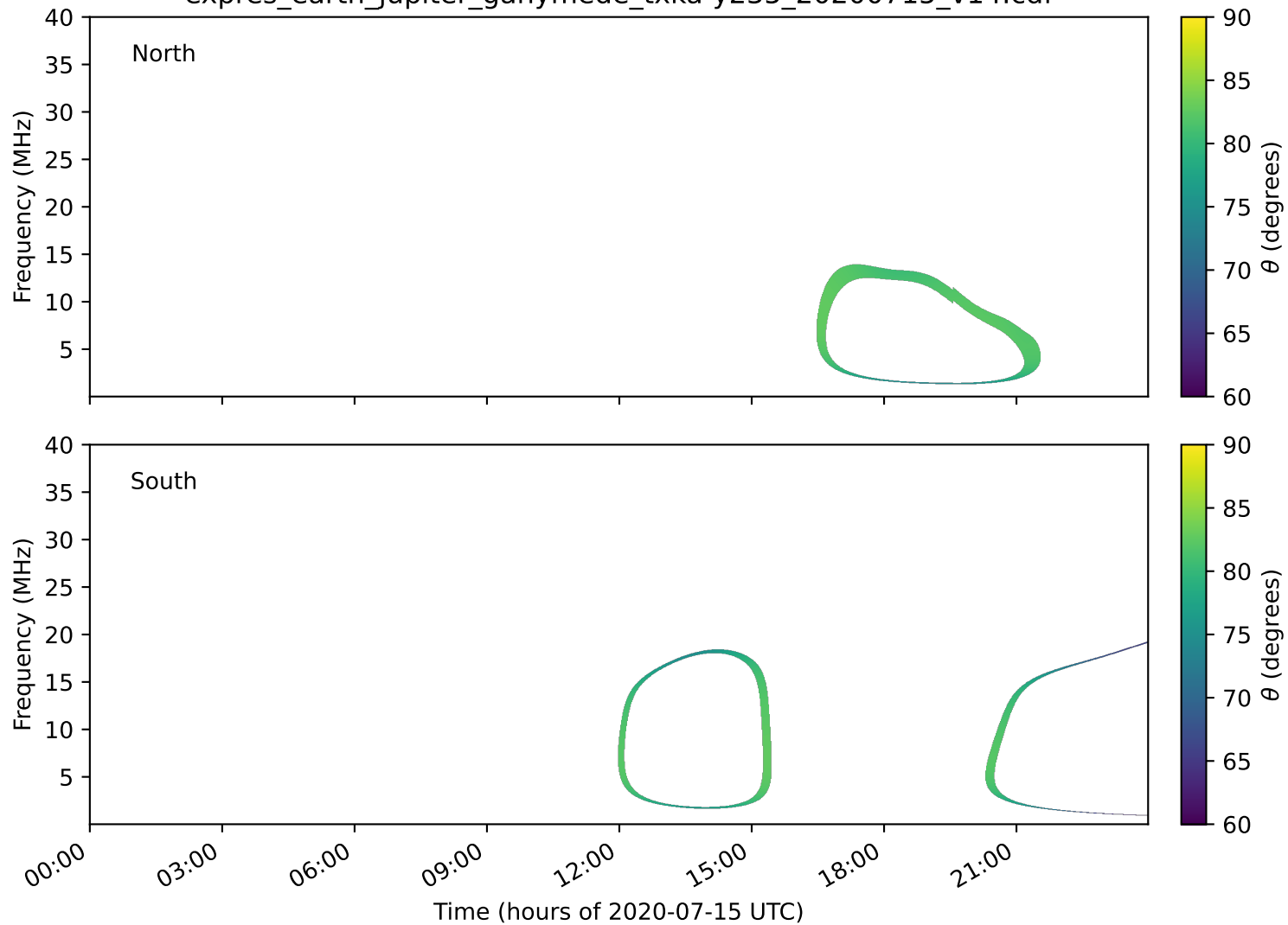
expres_earth_jupiter_ganymede_txka-y235_20200715_v14.cdf
