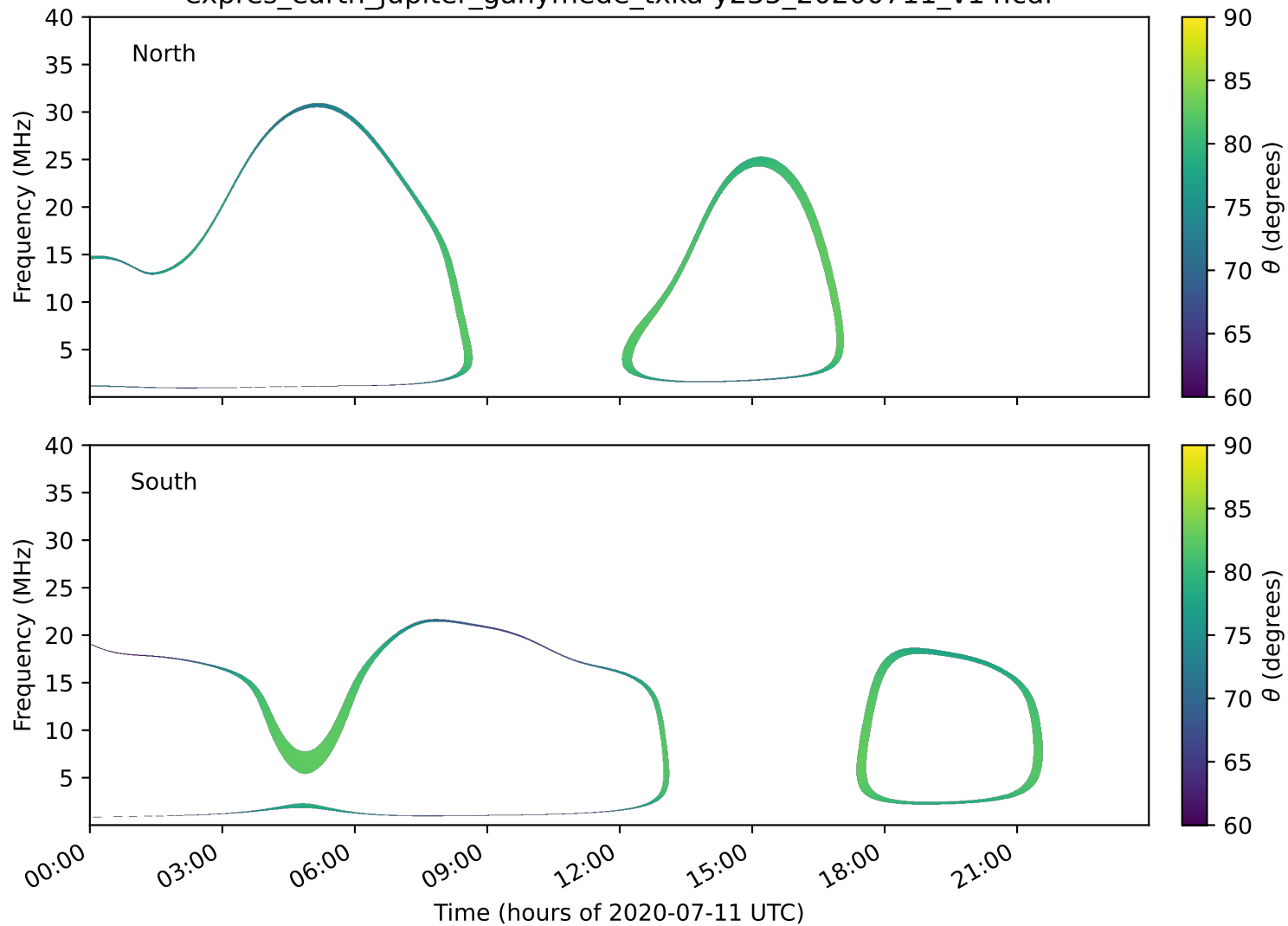
expres_earth_jupiter_ganymede_txka-y235_20200711_v14.cdf
