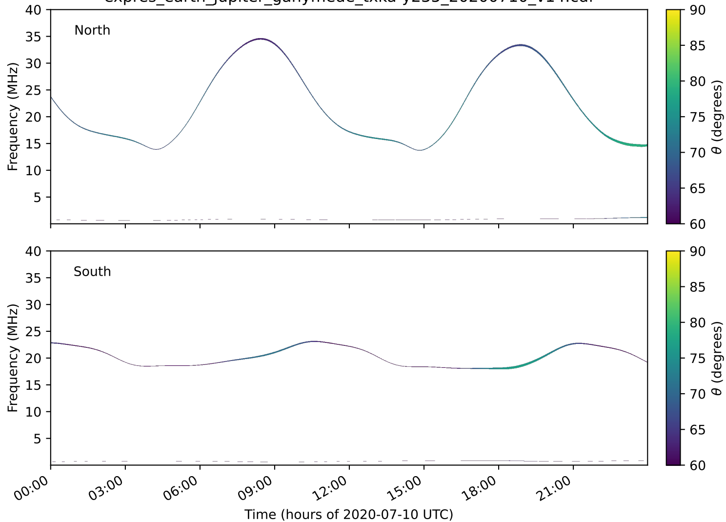
expres_earth_jupiter_ganymede_txka-y235_20200710_v14.cdf
