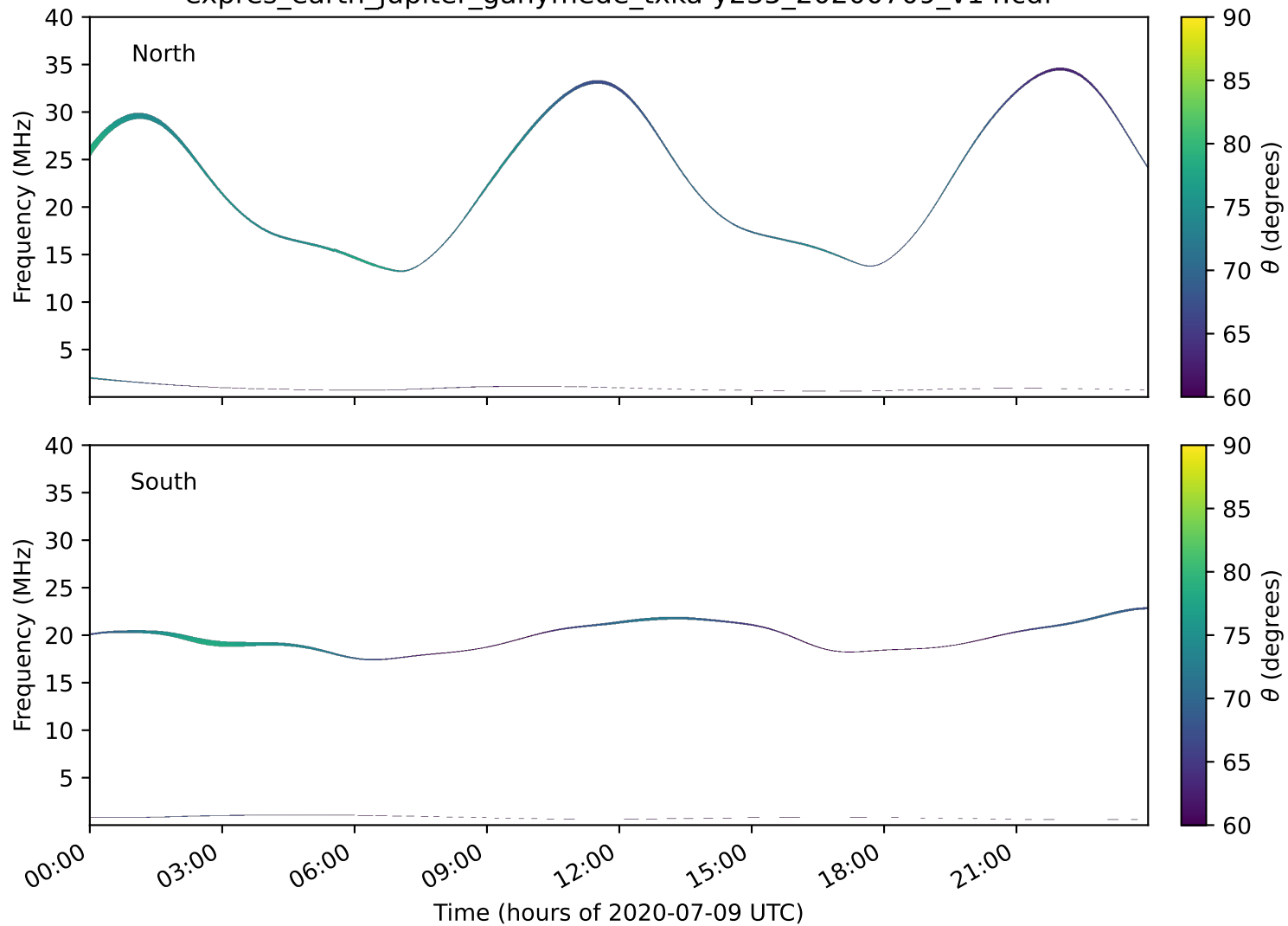
expres_earth_jupiter_ganymede_txka-y235_20200709_v14.cdf
