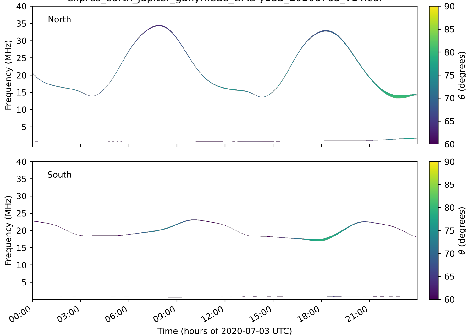
expres_earth_jupiter_ganymede_txka-y235_20200703_v14.cdf
