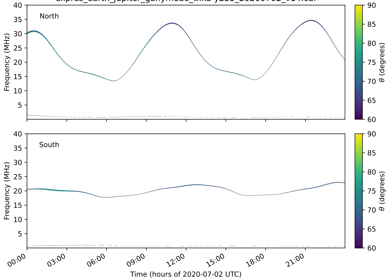
expres_earth_jupiter_ganymede_txka-y235_20200702_v14.cdf
