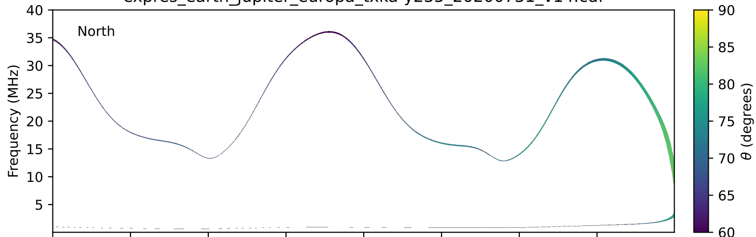
expres_earth_jupiter_europa_txka-y235_20200731_v14.cdf
