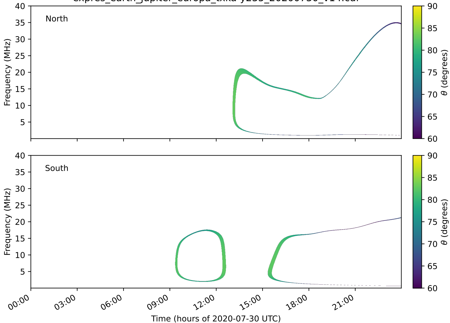
expres_earth_jupiter_europa_txka-y235_20200730_v14.cdf
