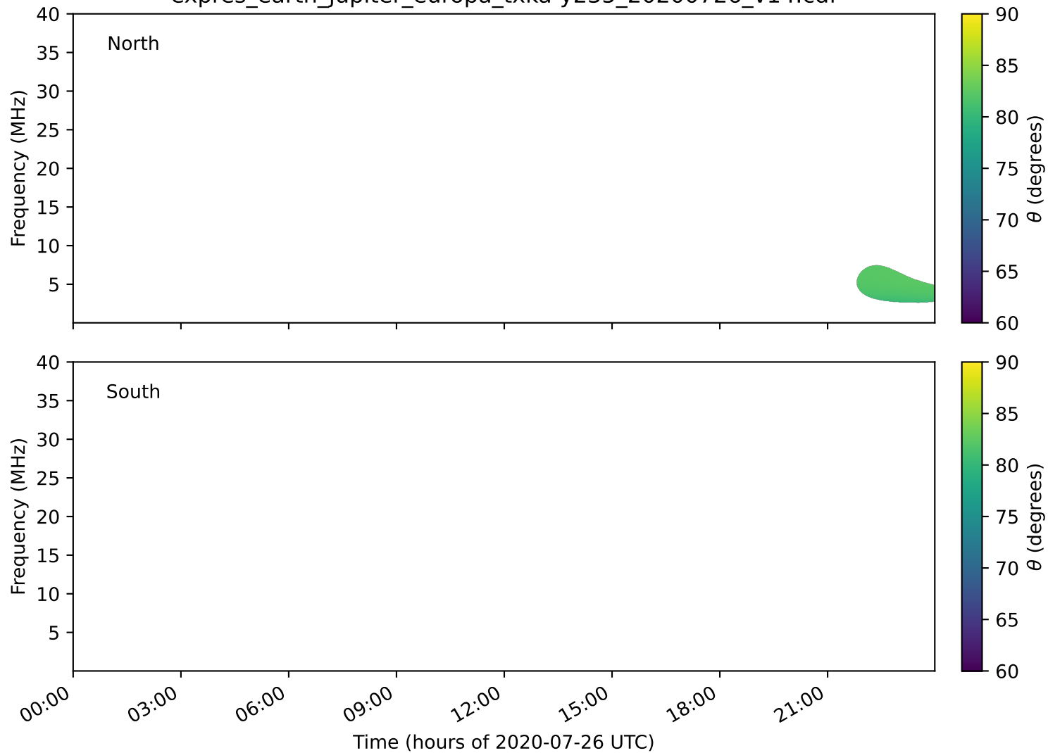
expres_earth_jupiter_europa_txka-y235_20200726_v14.cdf
