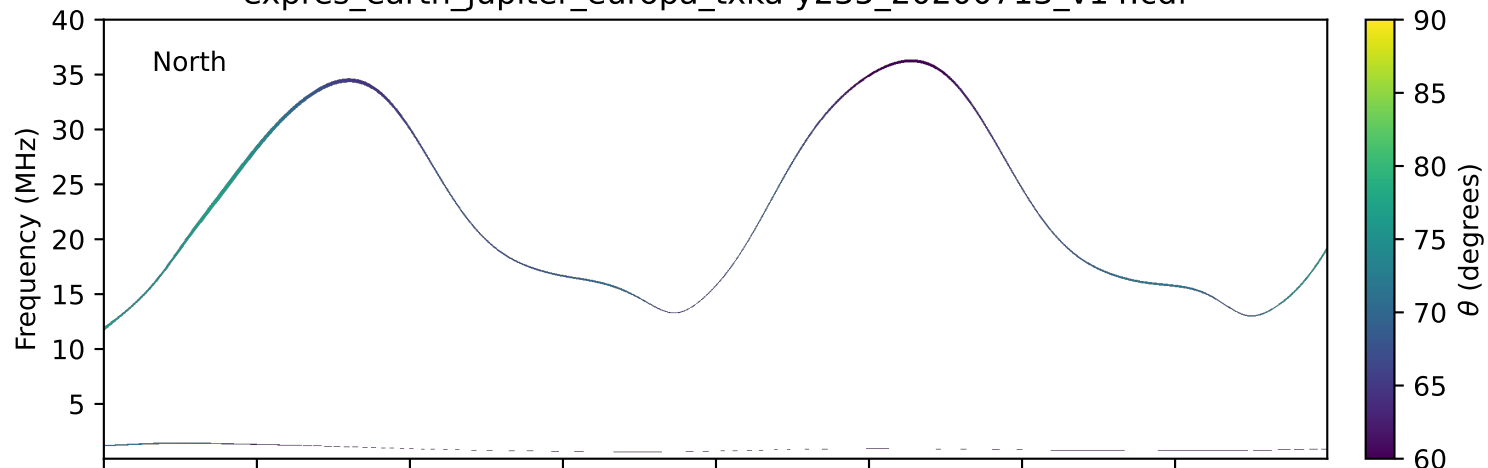
expres_earth_jupiter_europa_txka-y235_20200713_v14.cdf
