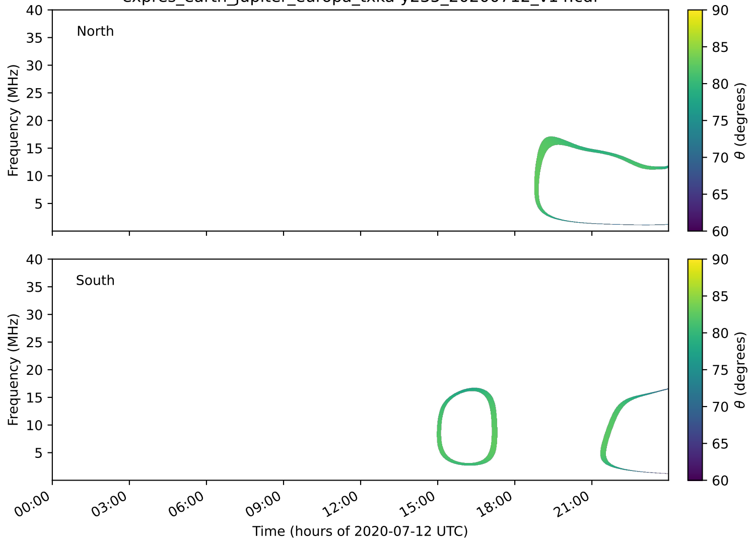
expres_earth_jupiter_europa_txka-y235_20200712_v14.cdf
