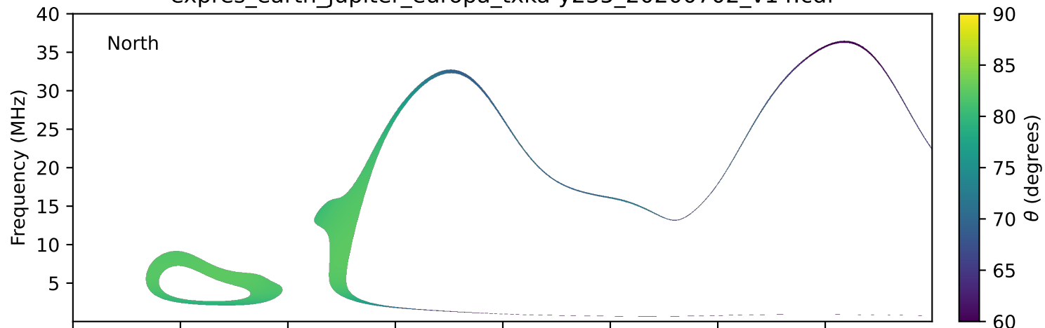
expres_earth_jupiter_europa_txka-y235_20200702_v14.cdf
