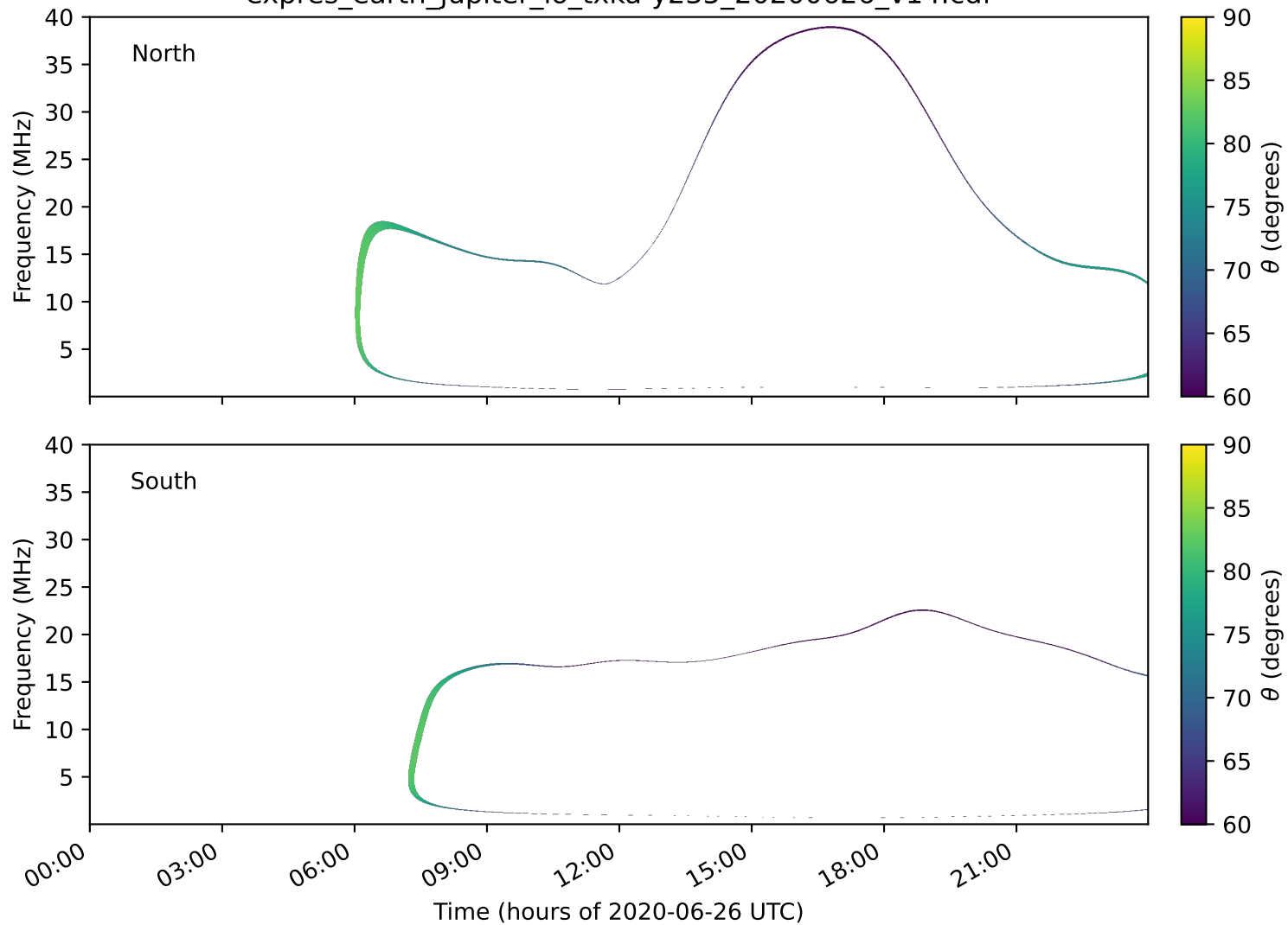
expres_earth_jupiter_io_txka-y235_20200626_v14.cdf
